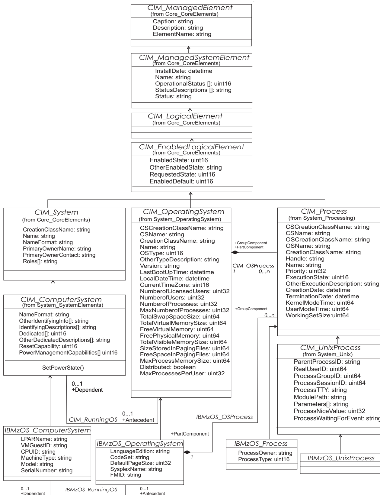
Figure 7: CIM Base classes extended by z/OS-specific classes (1)
